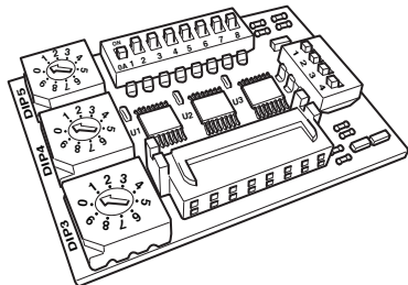
Fig. 35 Address and protocol board.
